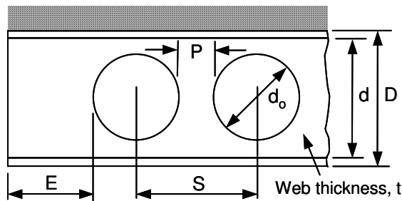
Figure 4.3 Geometric parameters for beams with web openings
