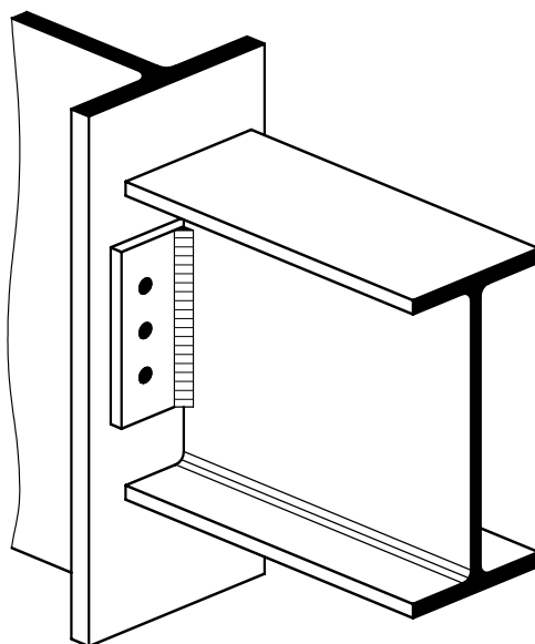
Figure 4.2 Flexible end plate beam-to-column connection
