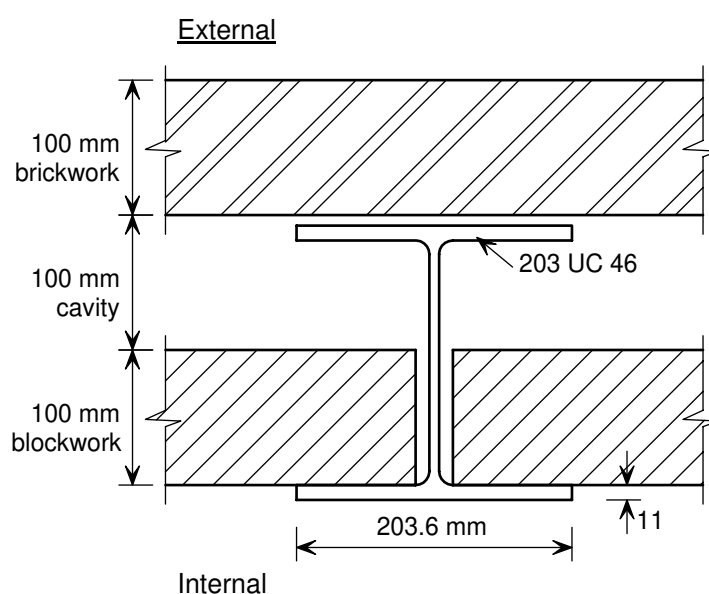
Figure 4.1 Column, partially protected by cavity wall construction.
